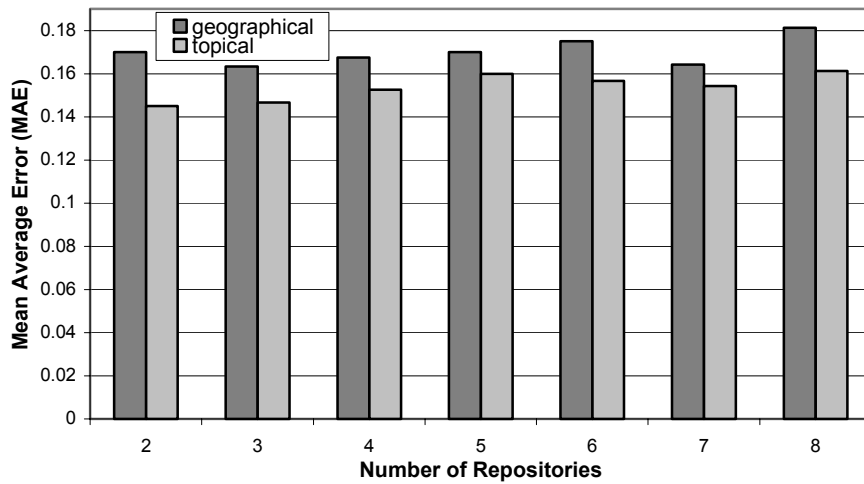
Figure 2, MAE vs. the number of repositories
